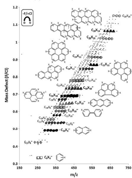
Figure 3. Mass defect plot of non-polar products produced in the thermal decomposition of PCTFE at 800 °C (X=Cl,F). Bold elemental compositions correspond to proposed X-PAH structures. Non-bold elemental compositions are proposed X-PAH fragment ions from chlorine loss or X-PAH molecular ions with an additional CF 2 group.
